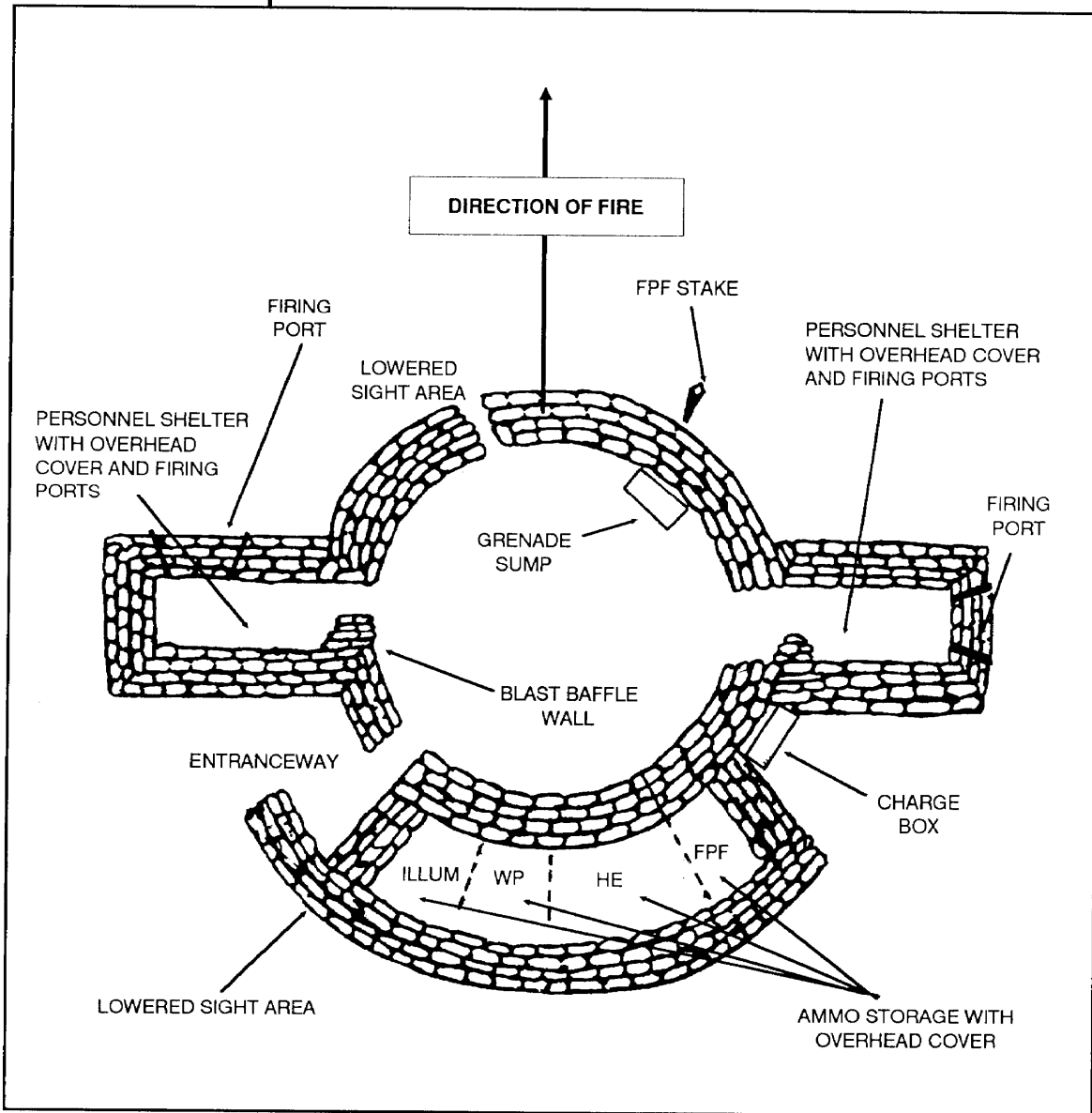
Figure 7-10. Completed dismantled mortar position (overhead view) with refinements.
